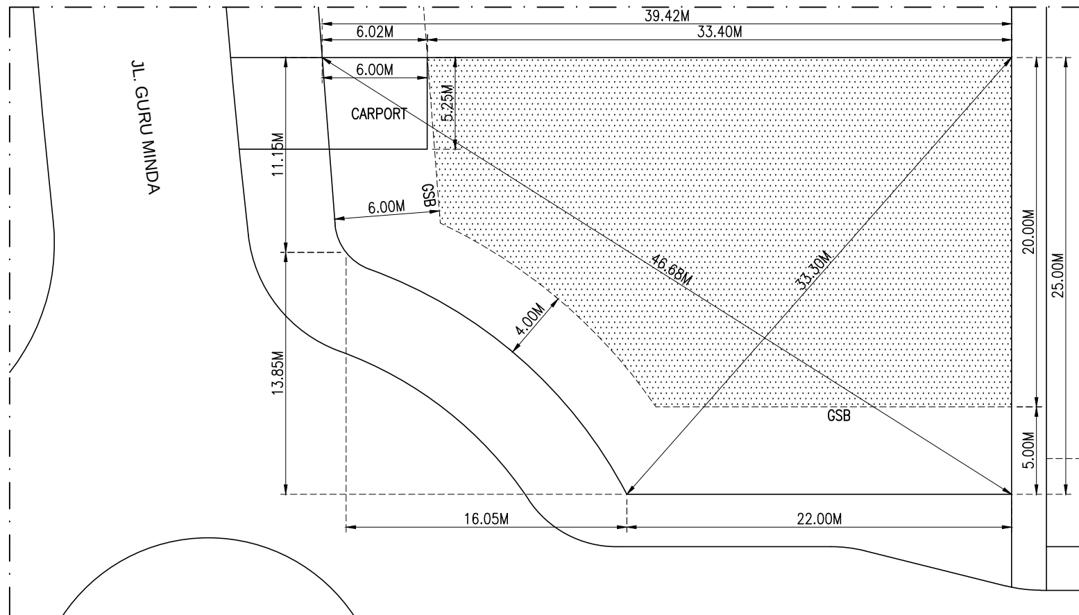
DENAH KAVLING JL. GURU MINDA NO. 85
